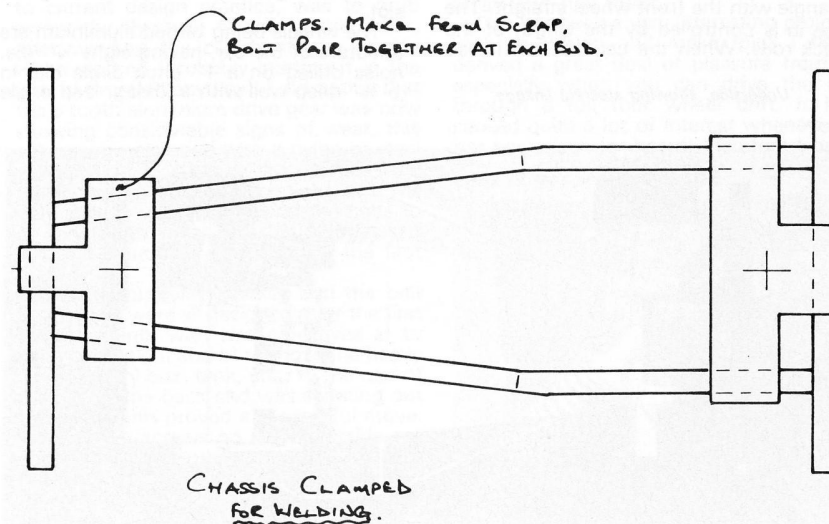
Below: Sketch showing clamps required for welding.
