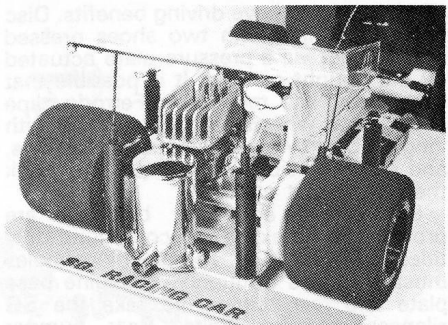
Rear end showing the silencer in place (drill your own holes) and also air filter — again SG.
