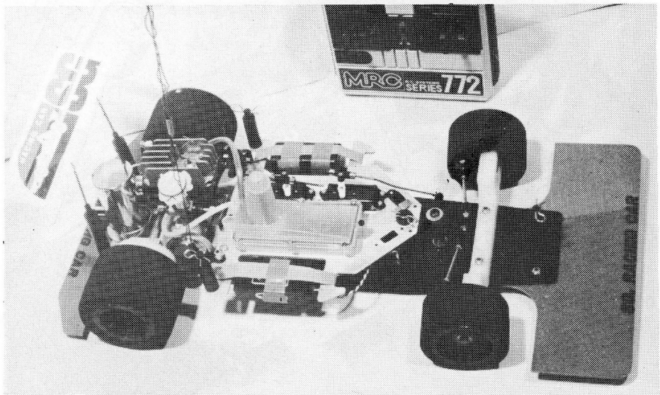
This shows the whole car with Tx in background — a most attractive and workmanlike assembly.
